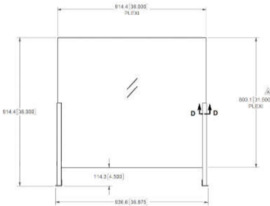
View 1. Elevation
